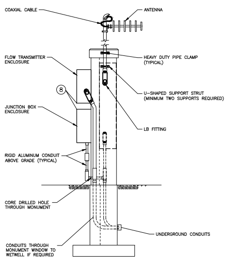
3 ELEVATION — CONTROL PANEL MONUMENT (SIDE) - N.T.S.
