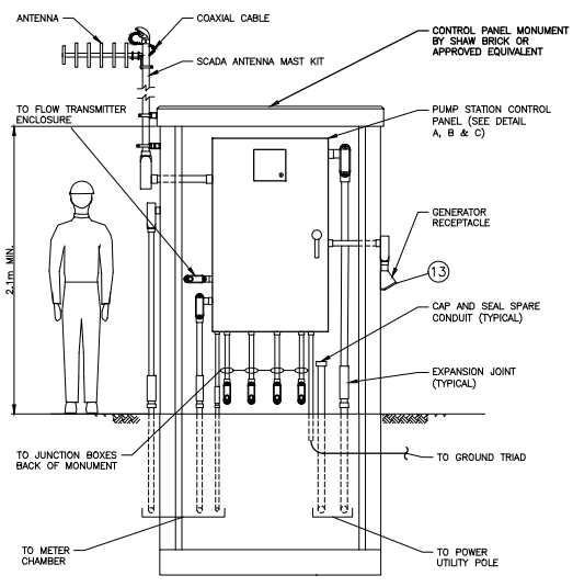
1 ELEVATION — CONTROL PANEL MONUMENT (FRONT) - N.T.S.
