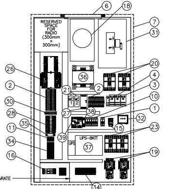
C DETAIL — CONTROL PANEL INTERIOR LAYOUT - N.T.S.
