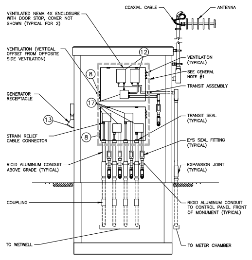
2 ELEVATION — CONTROL PANEL MONUMENT (BACK) - N.T.S.
