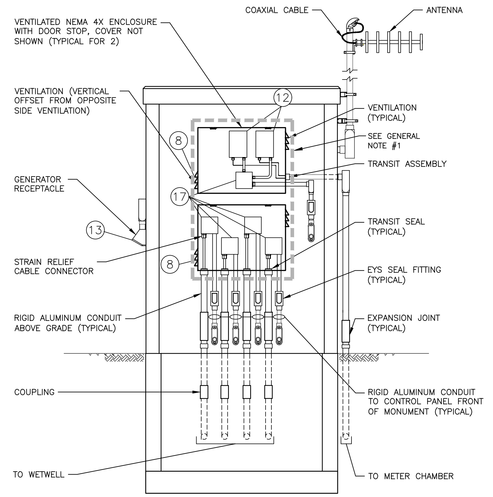
2 ELEVATION — CONTROL PANEL MONUMENT (BACK) N.T.S.
