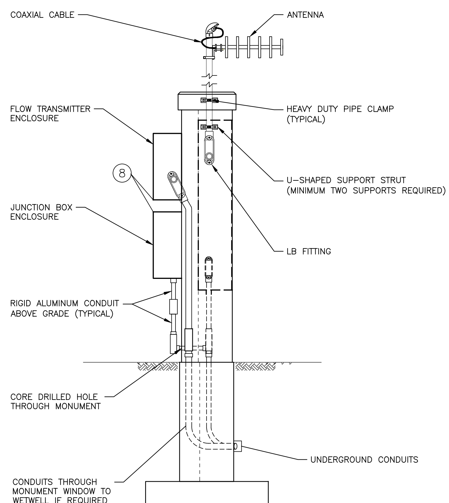
3 ELEVATION — CONTROL PANEL MONUMENT (SIDE) N.T.S.
