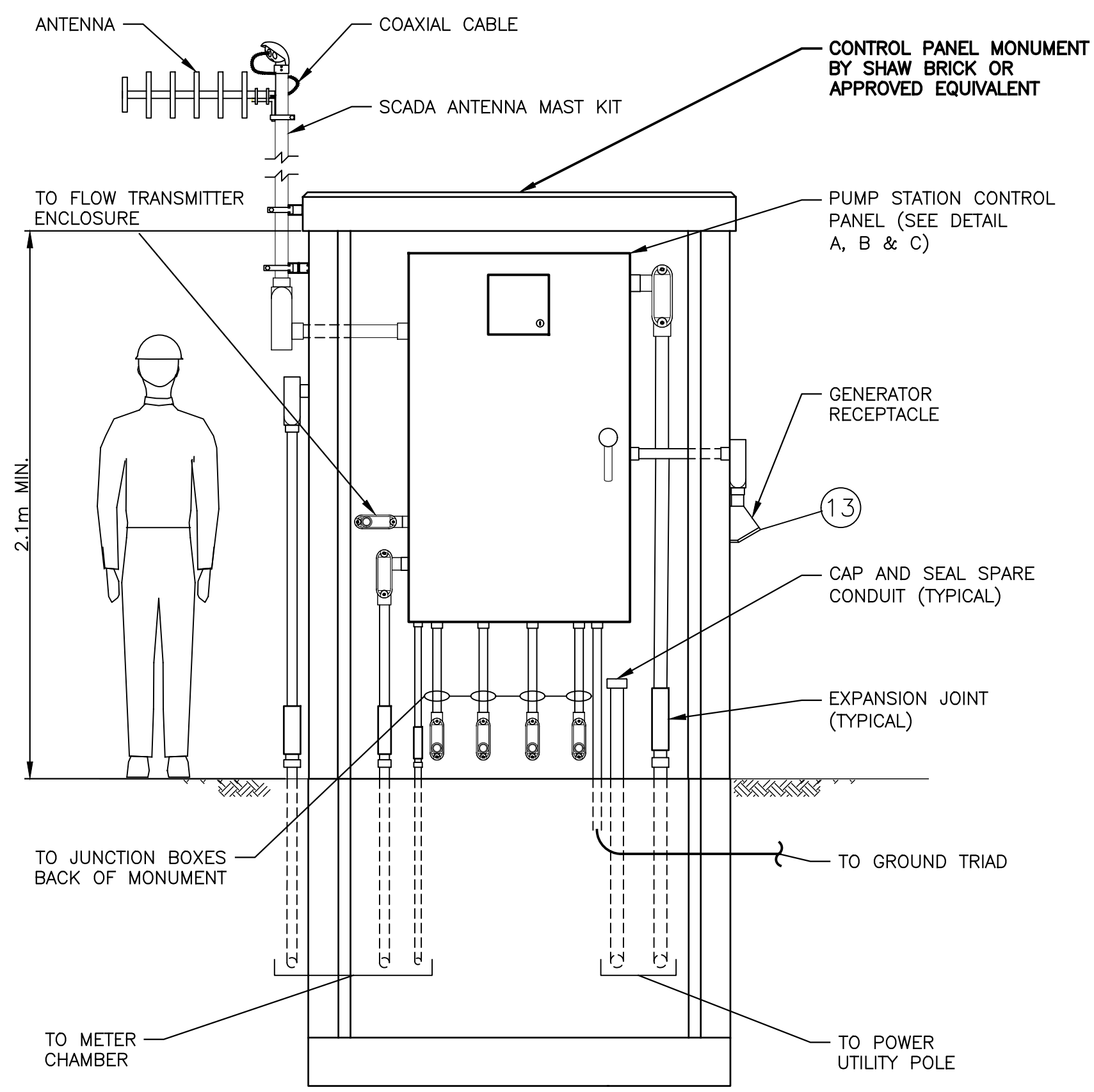
1 ELEVATION — CONTROL PANEL MONUMENT (FRONT) N.T.S.
