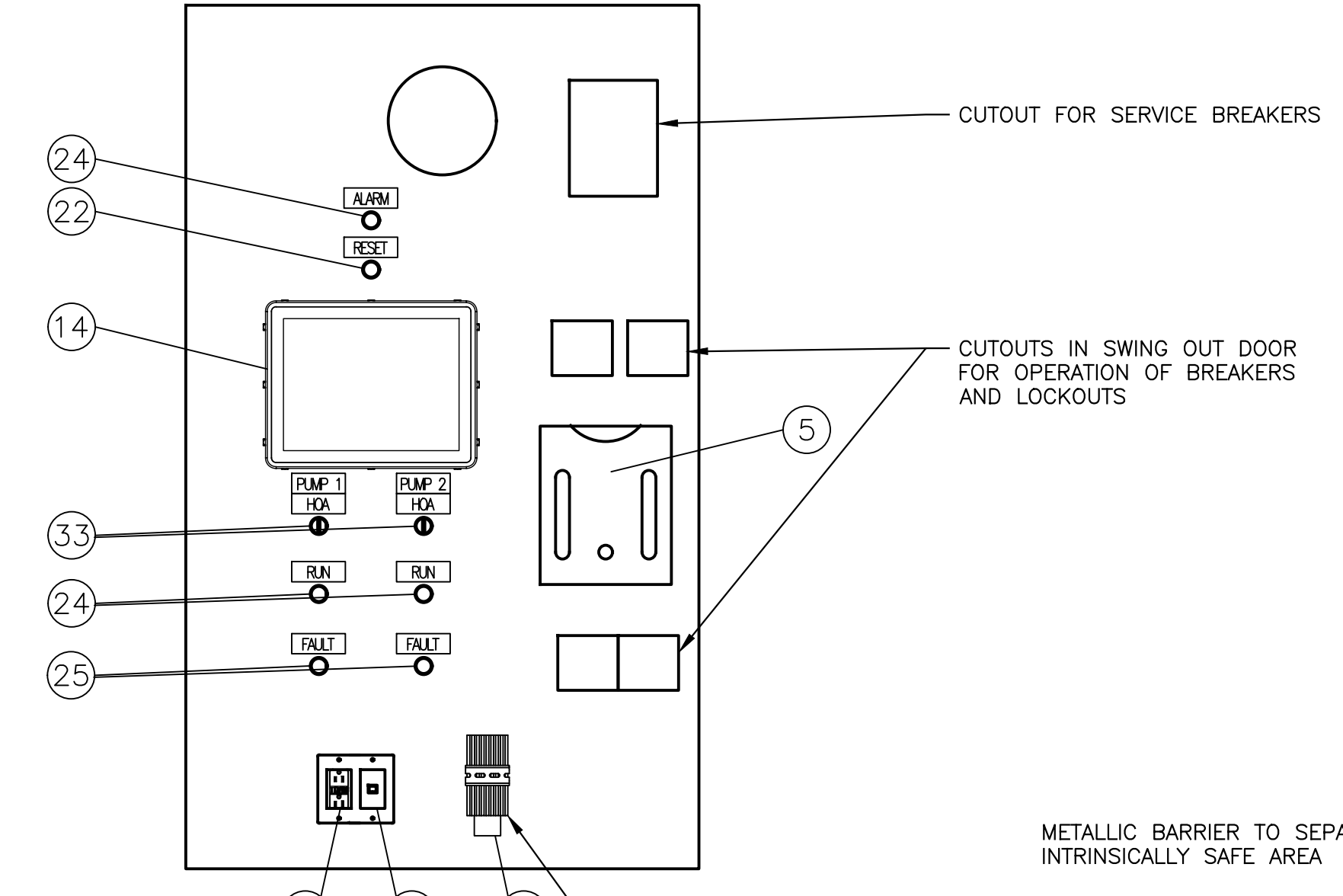
B DETAIL— CONTROL PANEL SWING OUT DOOR LAYOUT N.T.S.
