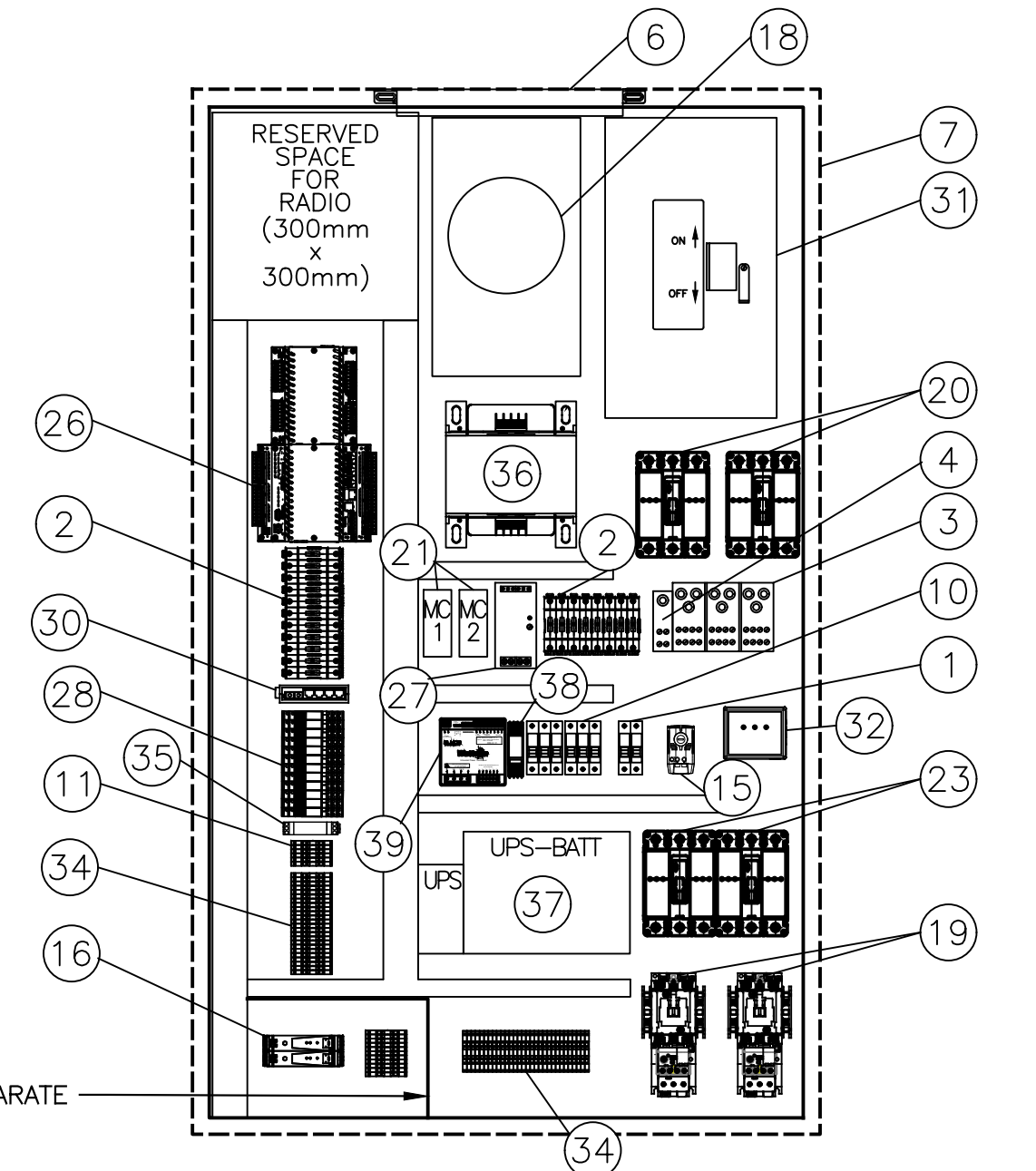
C DETAIL— CONTROL PANEL INTERIOR LAYOUT N.T.S.
