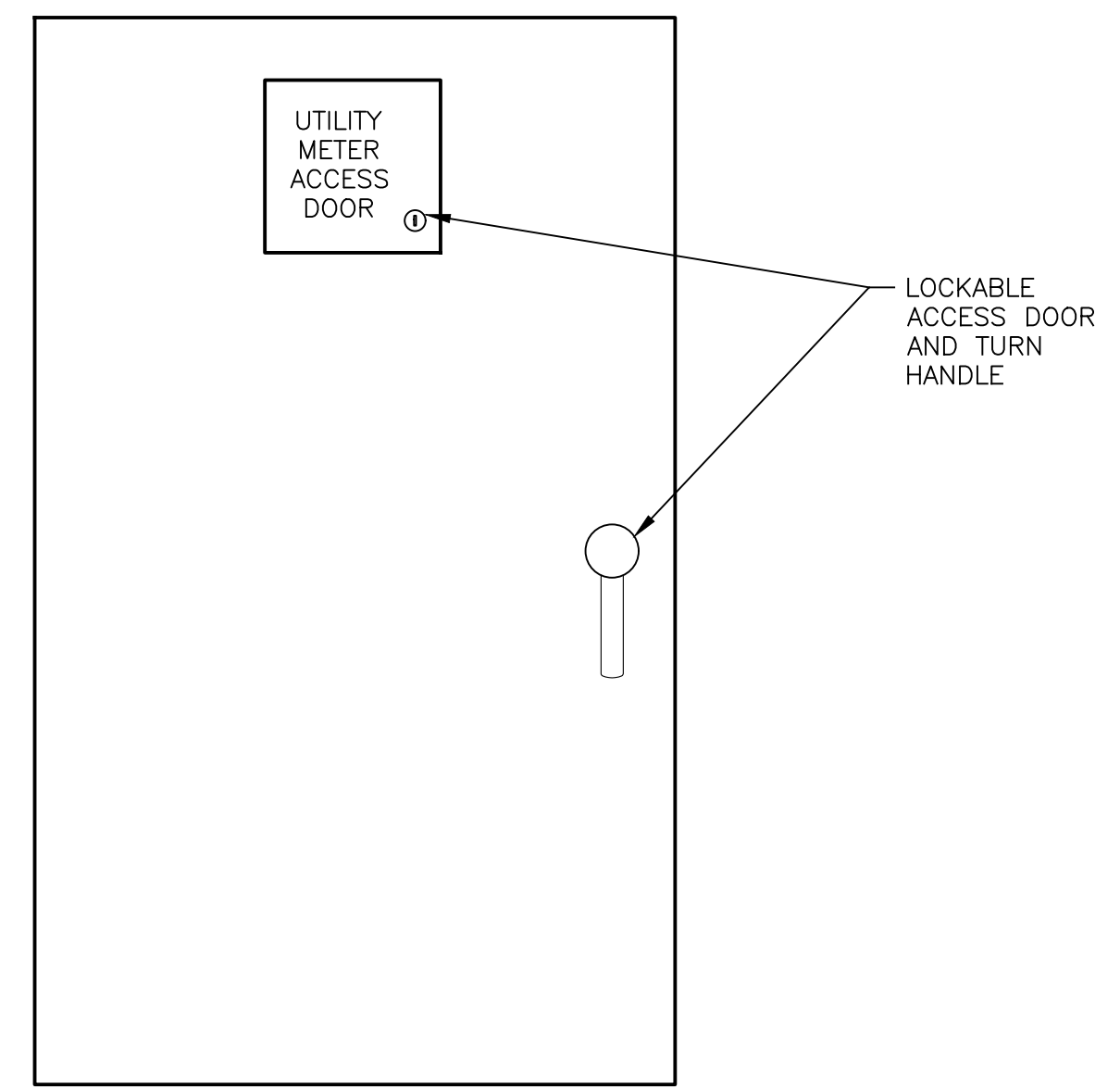
A DETAIL— CONTROL PANEL FRONT DOOR N.T.S.
