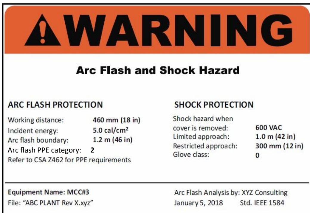
Figure 4.1 - Example of an Arc Flash and Shock Warning Label
